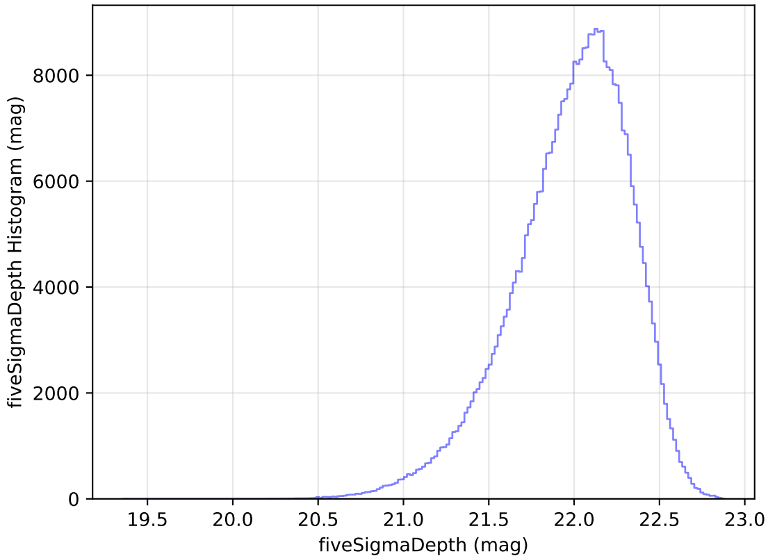
too_ignore_10_1v3.4_10yrs All sky y band: fiveSigmaDepth Histogram
