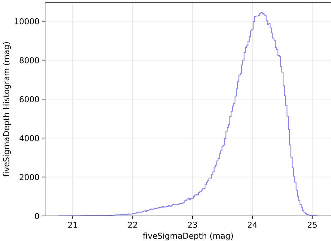
too_ignore_10_1v3.4_10yrs All sky r band: fiveSigmaDepth Histogram
