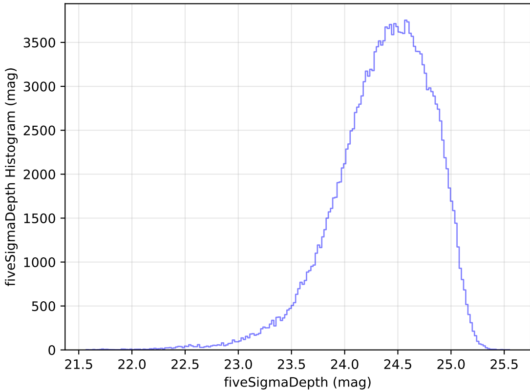
too_ignore_10_1v3.4_10yrs All sky g band: fiveSigmaDepth Histogram
