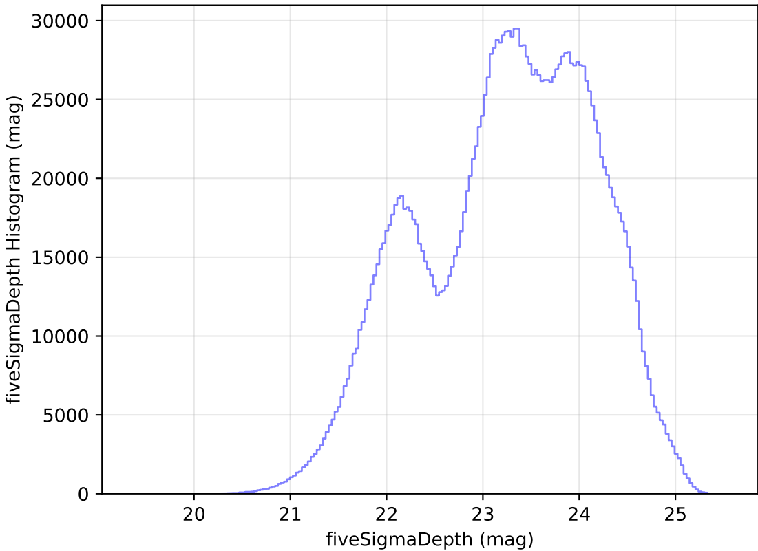
too_ignore_10_1v3.4_10yrs All sky all bands: fiveSigmaDepth Histogram
