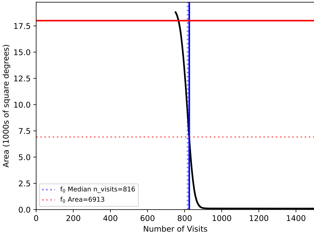
too_ignore_10_1v3.4_10yrs WFD: f0
