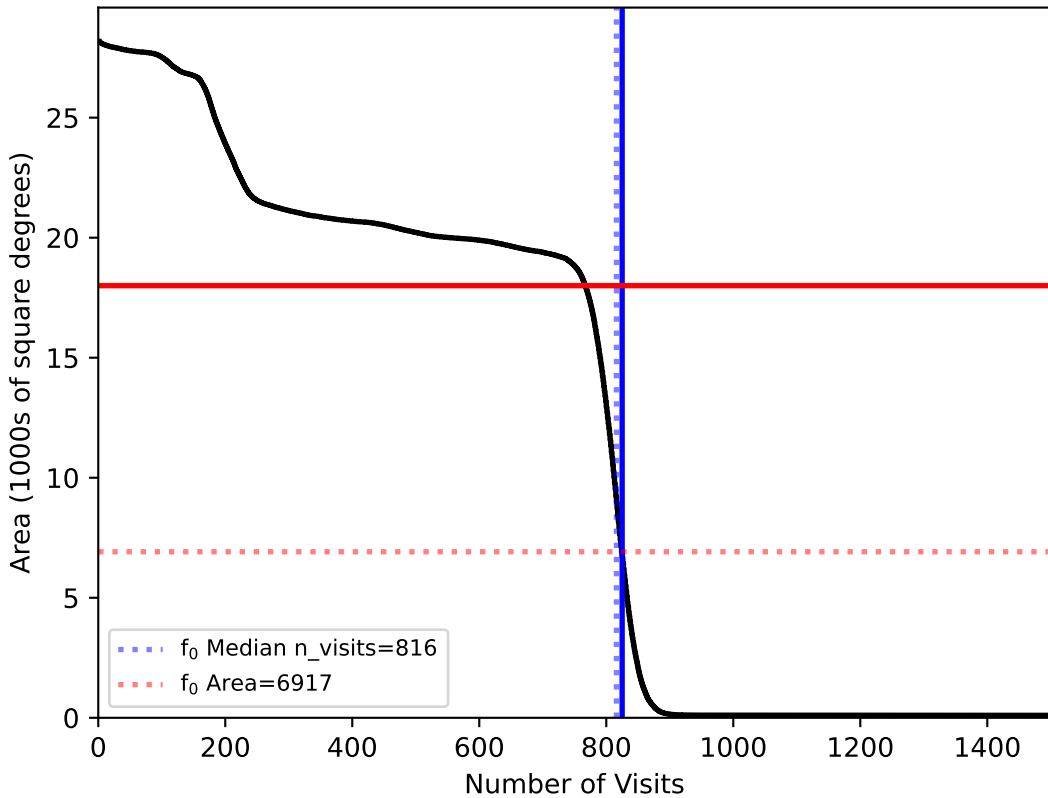
too_ignore_10_1v3.4_10yrs All sky: f0
