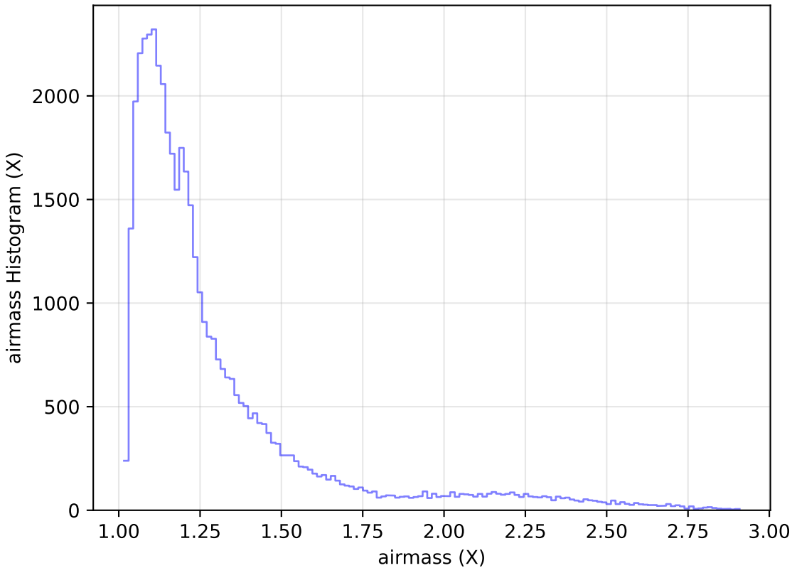
too_ignore_10_1v3.4_10yrs Yr 1 z band: airmass Histogram
