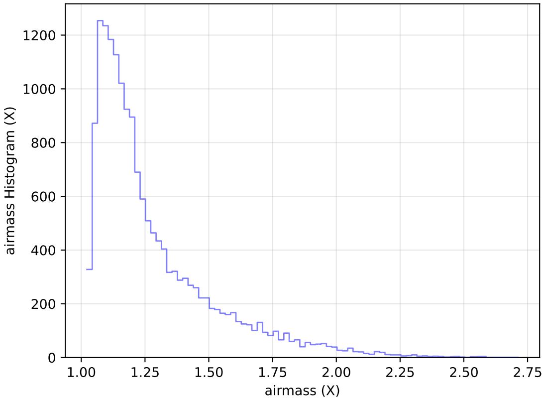
too_ignore_10_1v3.4_10yrs Yr 1 u band: airmass Histogram
