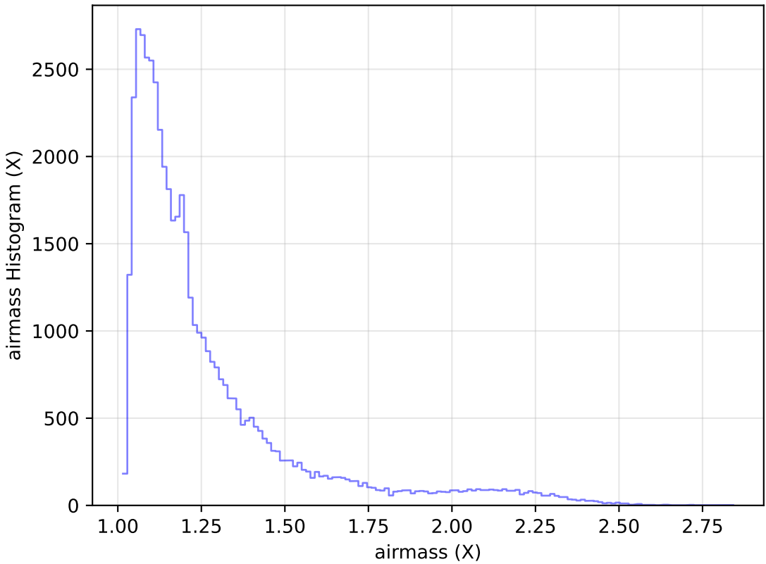
too_ignore_10_1v3.4_10yrs Yr 1 r band: airmass Histogram
