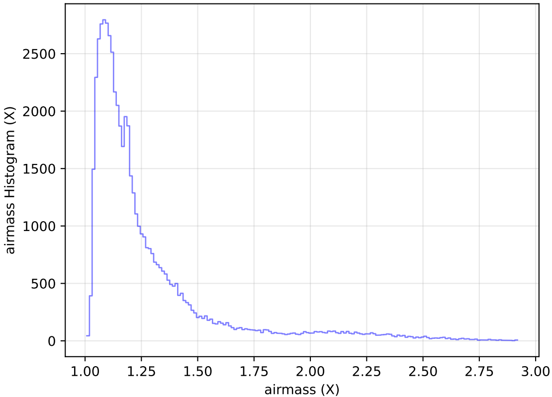
too_ignore_10_1v3.4_10yrs Yr 1 i band: airmass Histogram
