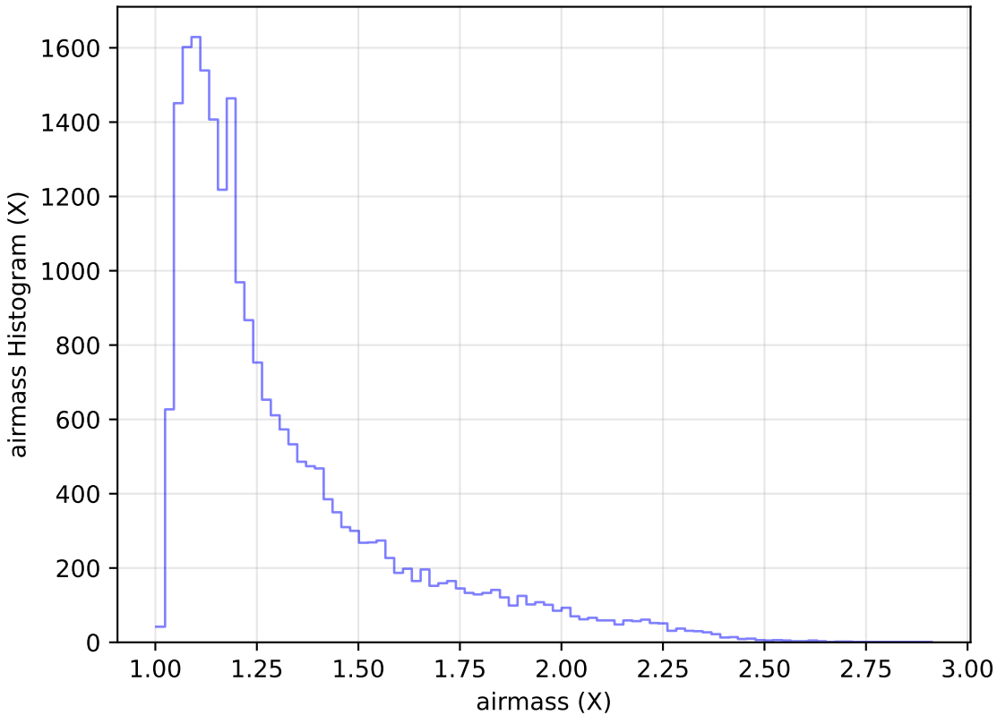
too_ignore_10_1v3.4_10yrs Yr 1 g band: airmass Histogram
