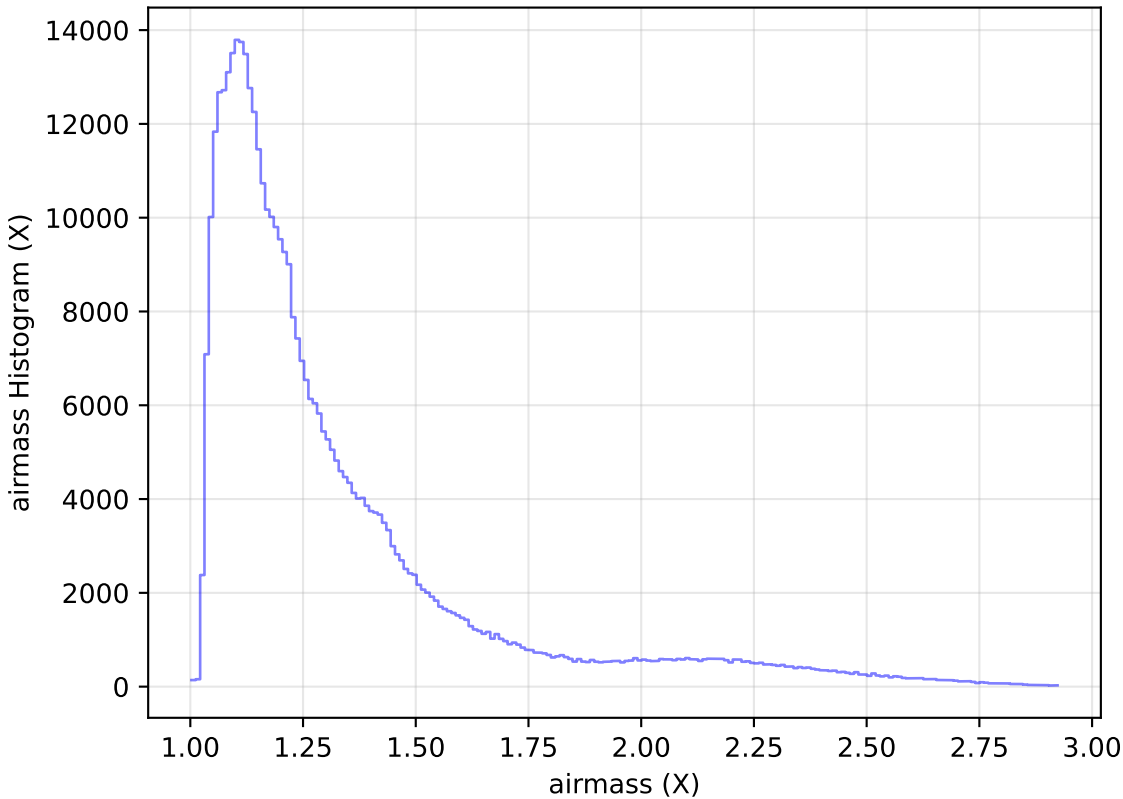
too_ignore_10_1v3.4_10yrs WFD z band: airmass Histogram
