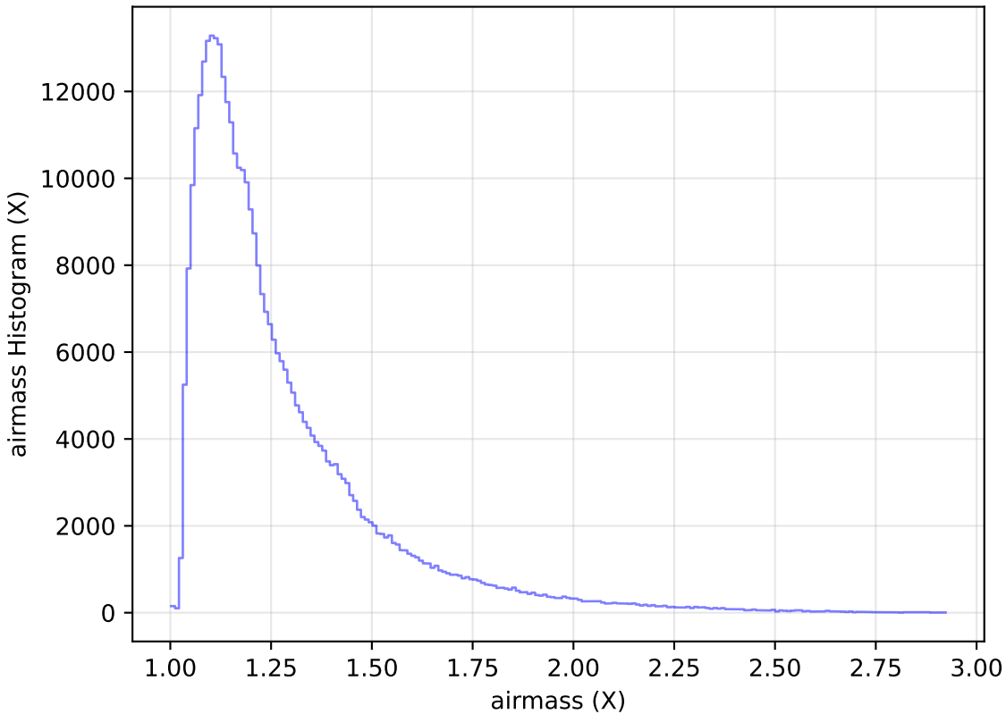
too_ignore_10_1v3.4_10yrs WFD y band: airmass Histogram
