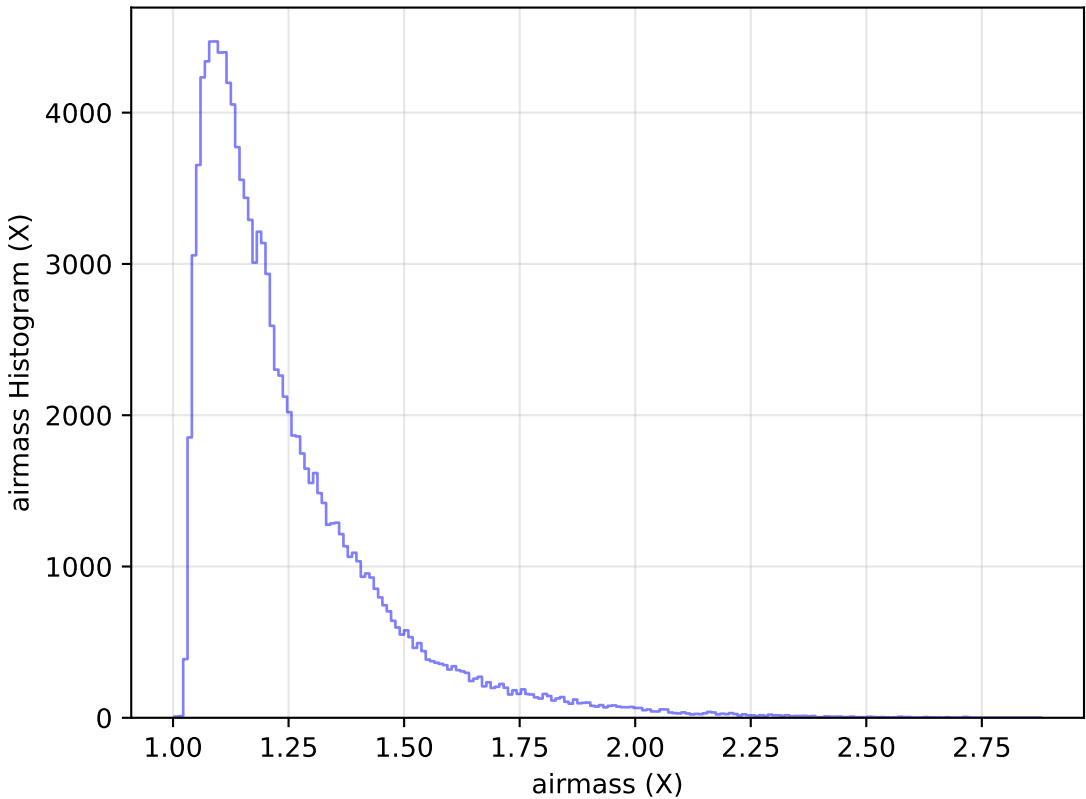
too_ignore_10_1v3.4_10yrs WFD u band: airmass Histogram
