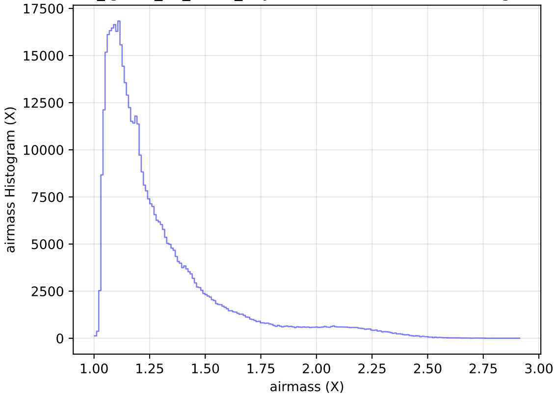
too_ignore_10_1v3.4_10yrs WFD r band: airmass Histogram
