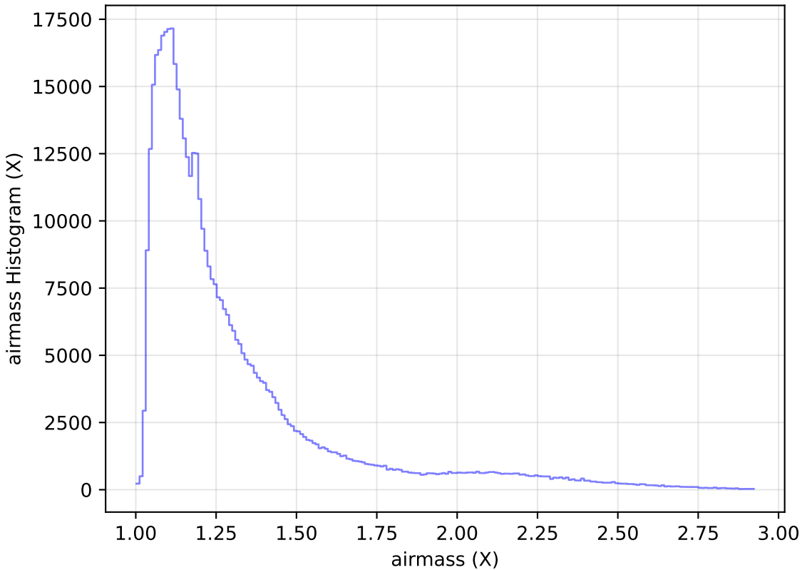
too_ignore_10_1v3.4_10yrs WFD i band: airmass Histogram
