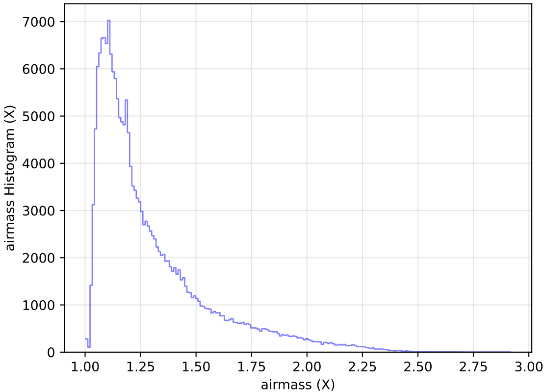
too_ignore_10_1v3.4_10yrs WFD g band: airmass Histogram
