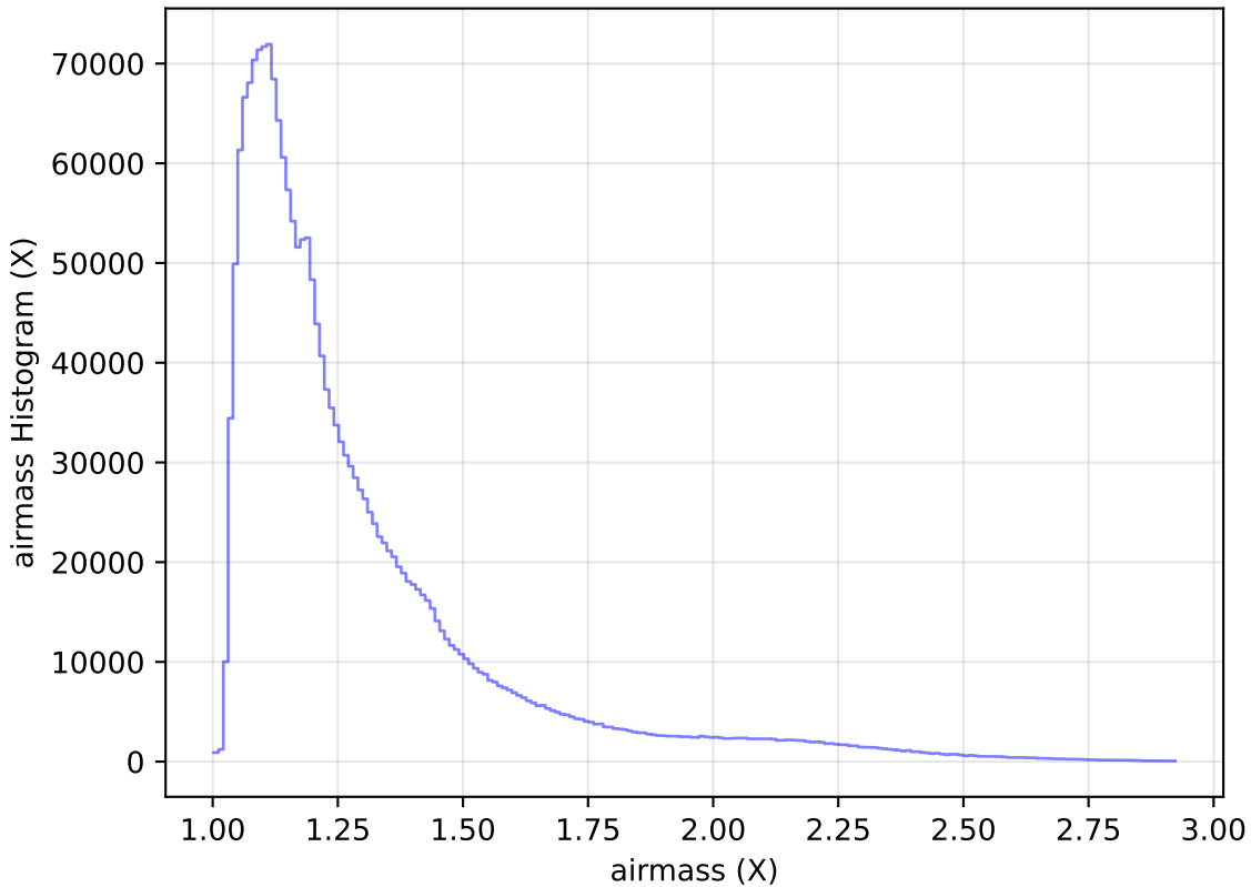
too_ignore_10_1v3.4_10yrs WFD all bands: airmass Histogram
