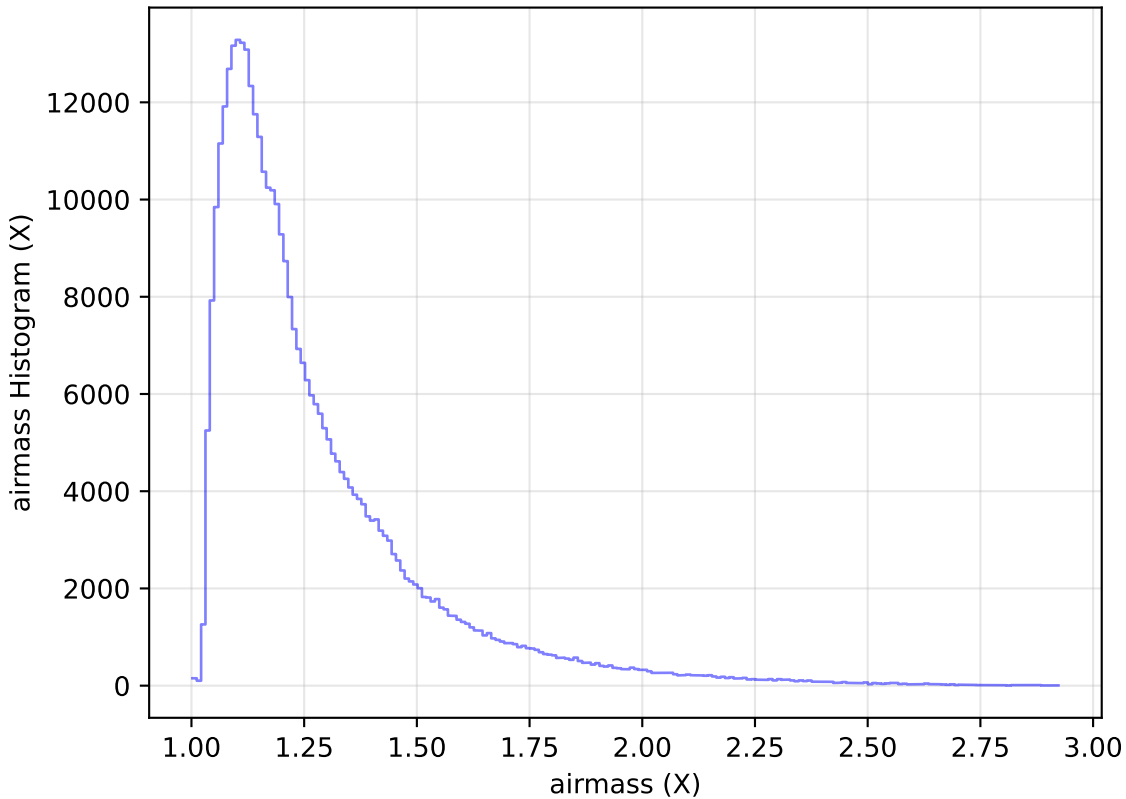
too_ignore_10_1v3.4_10yrs All sky y band: airmass Histogram
