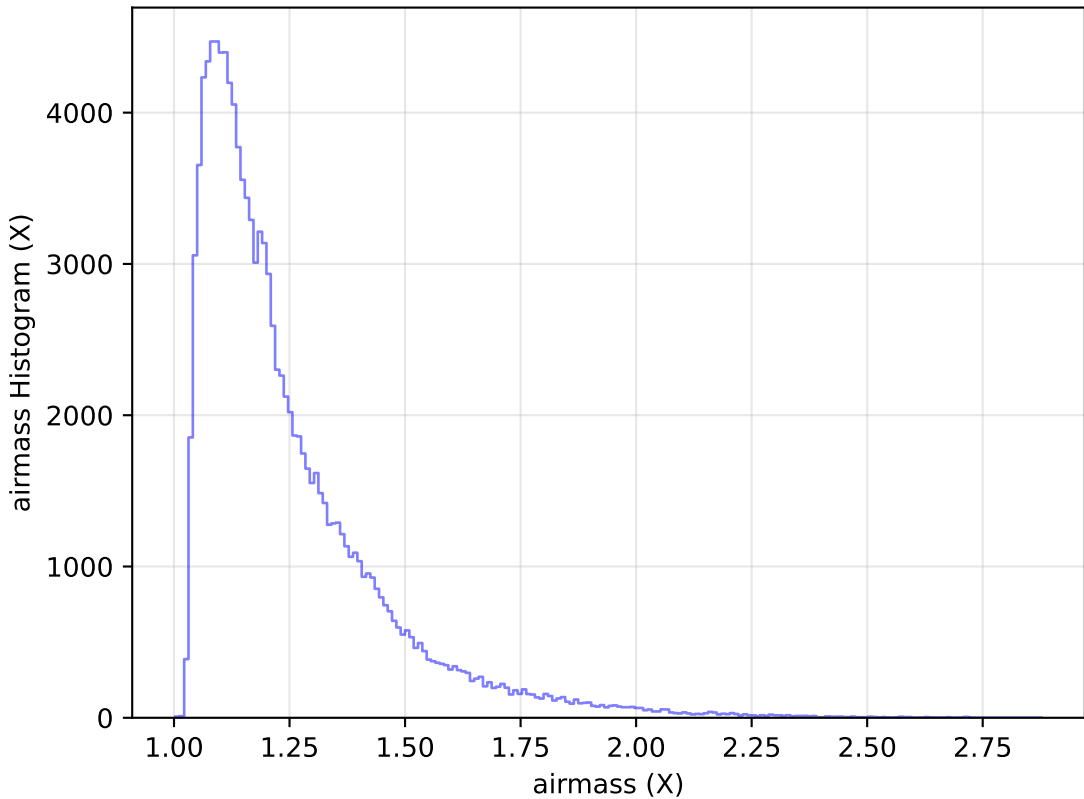
too_ignore_10_1v3.4_10yrs All sky u band: airmass Histogram
