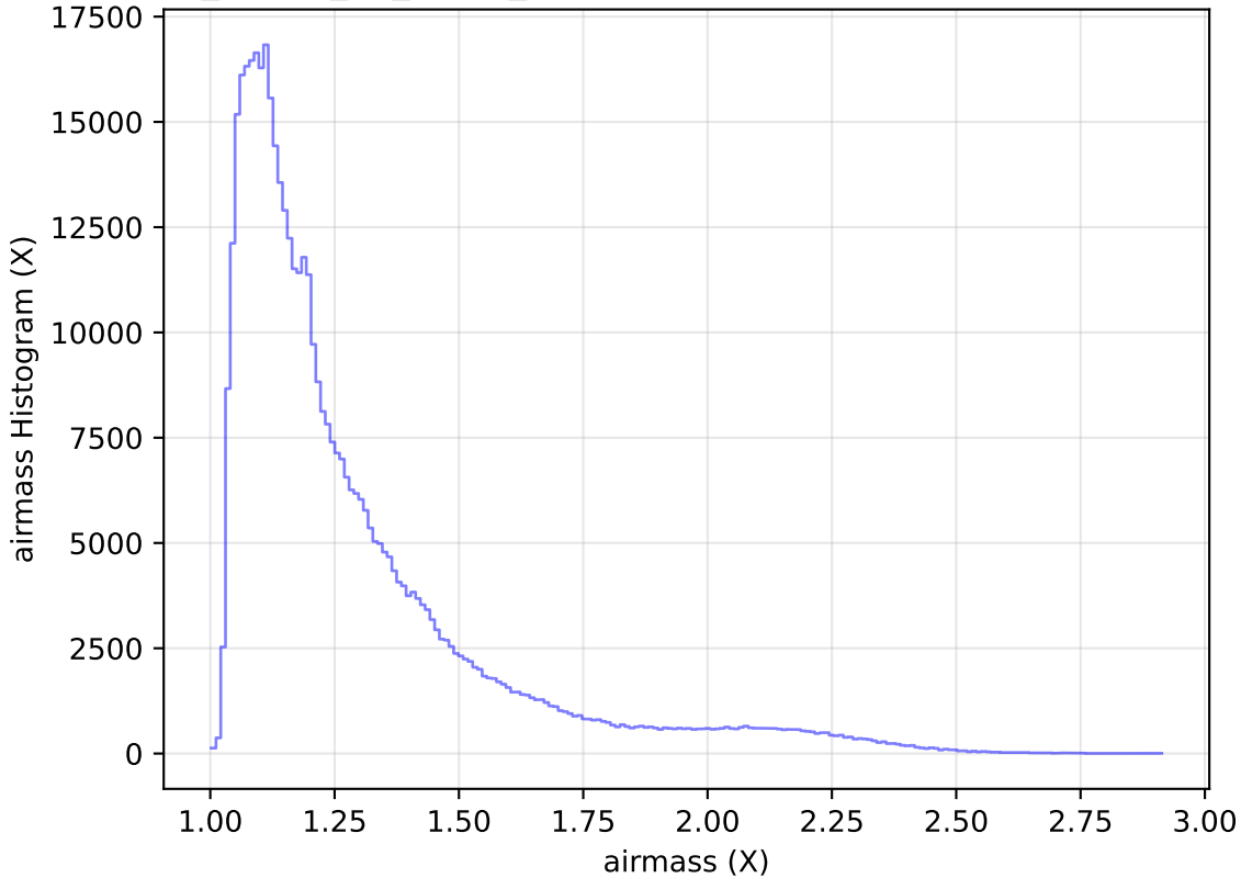
too_ignore_10_1v3.4_10yrs All sky r band: airmass Histogram
