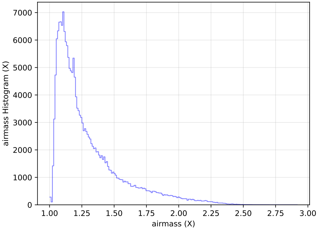
too_ignore_10_1v3.4_10yrs All sky g band: airmass Histogram
