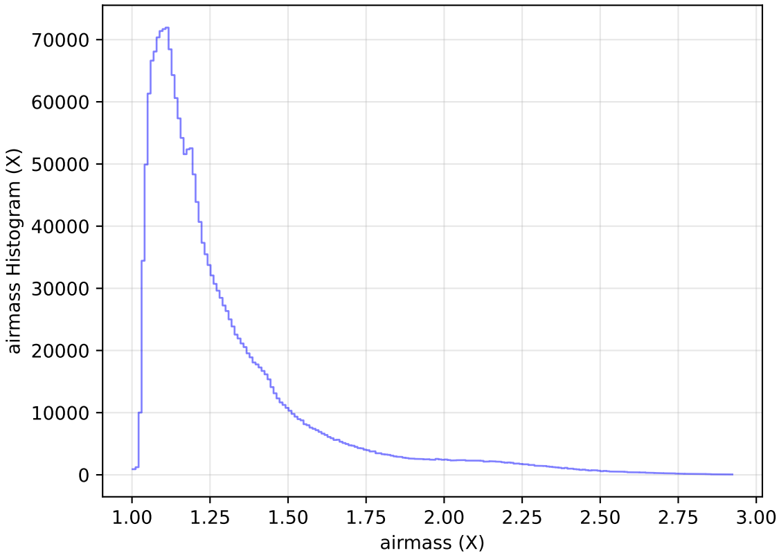
too_ignore_10_1v3.4_10yrs All sky all bands: airmass Histogram
