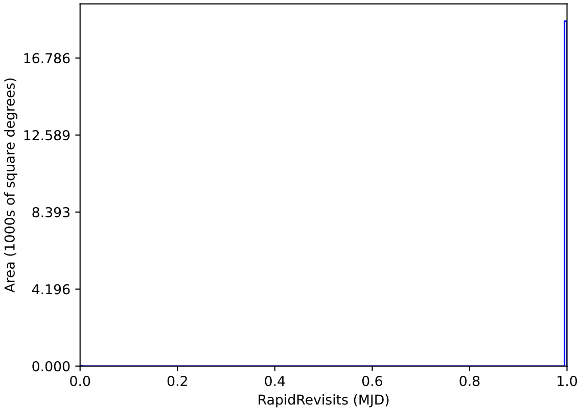
too_ignore_10_1v3.4_10yrs WFD: RapidRevisits
