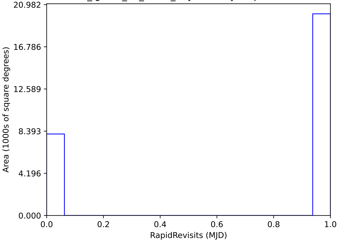
too_ignore_10_1v3.4_10yrs All sky: RapidRevisits
