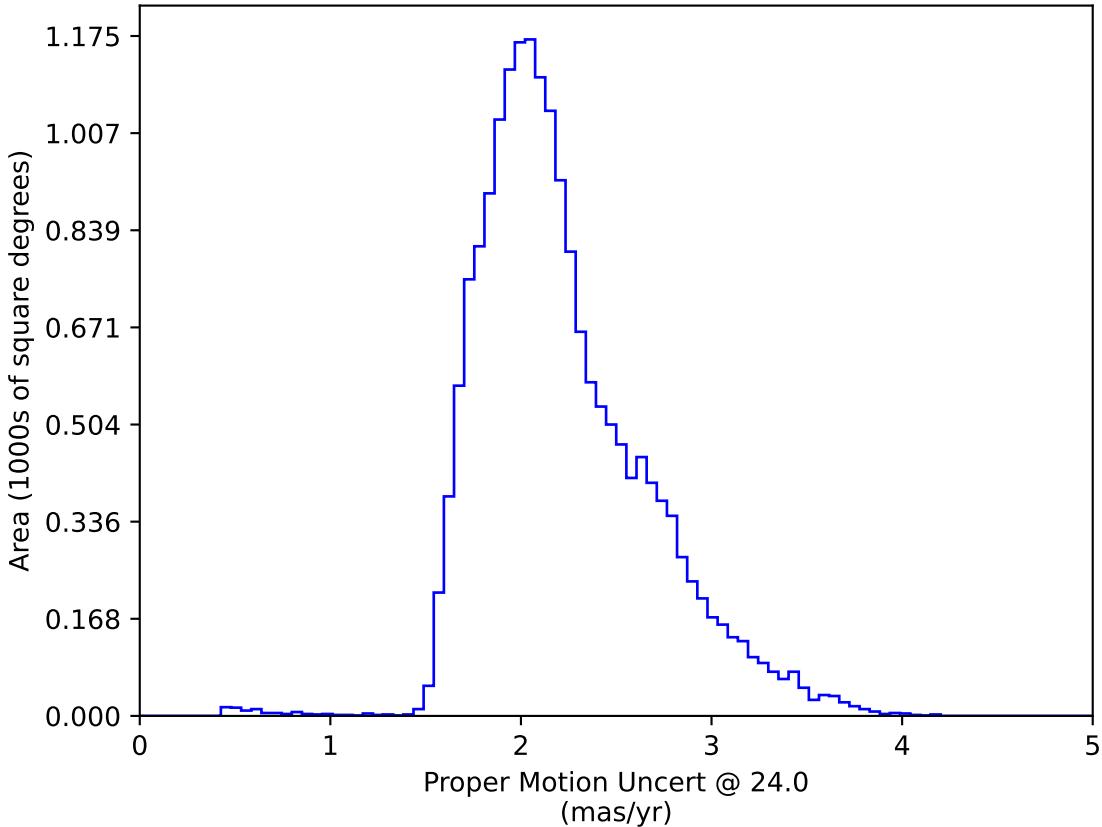
too_ignore_10_1v3.4_10yrs WFD: Proper Motion Uncert @ 24.0
