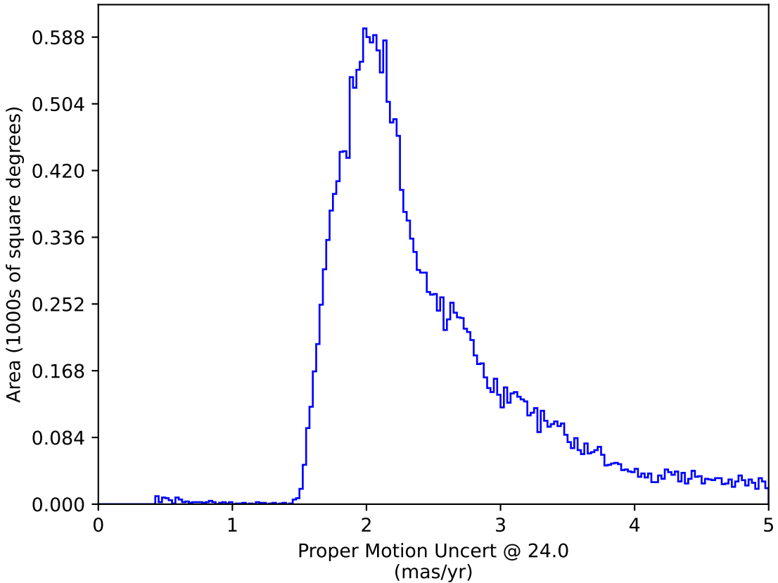
too_ignore_10_1v3.4_10yrs All sky: Proper Motion Uncert @ 24.0
