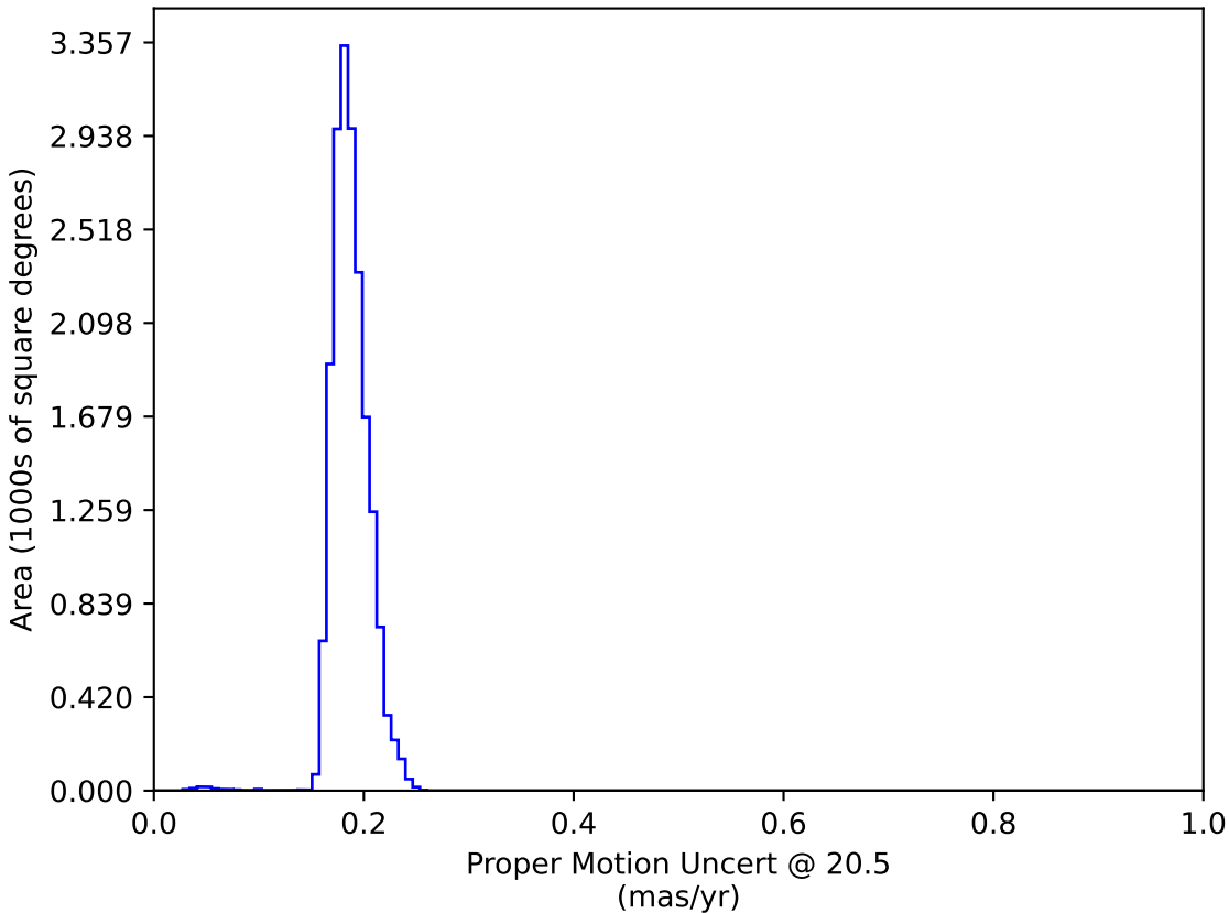
too_ignore_10_1v3.4_10yrs WFD: Proper Motion Uncert @ 20.5
