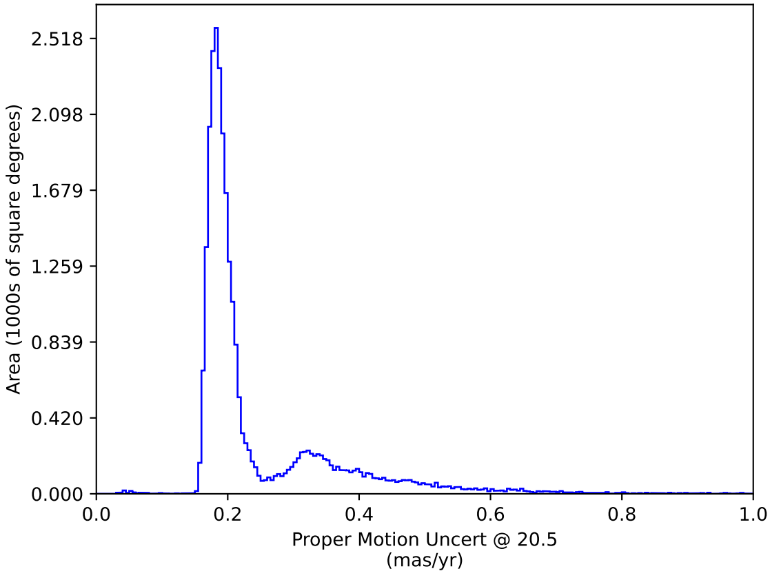
too_ignore_10_1v3.4_10yrs All sky: Proper Motion Uncert @ 20.5
