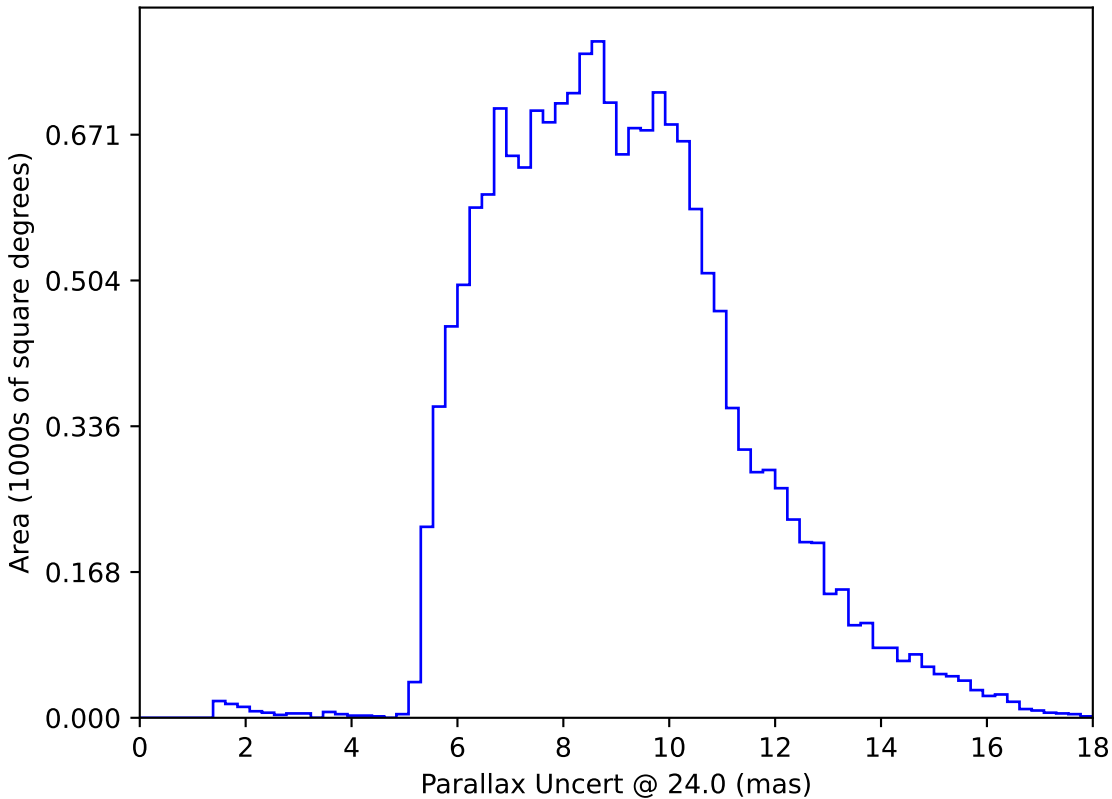
too_ignore_10_1v3.4_10yrs WFD: Parallax Uncert @ 24.0
