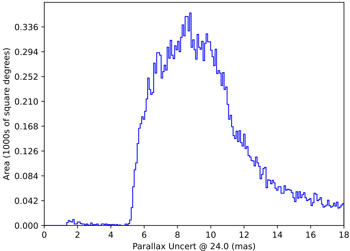
too_ignore_10_1v3.4_10yrs All sky: Parallax Uncert @ 24.0
