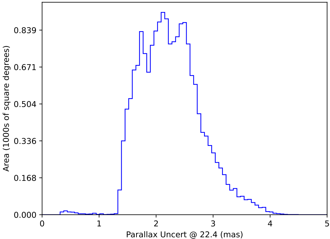
too_ignore_10_1v3.4_10yrs WFD: Parallax Uncert @ 22.4
