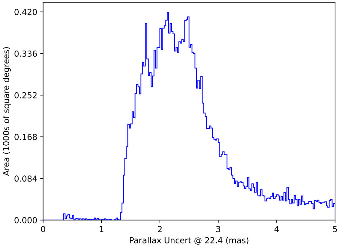
too_ignore_10_1v3.4_10yrs All sky: Parallax Uncert @ 22.4
