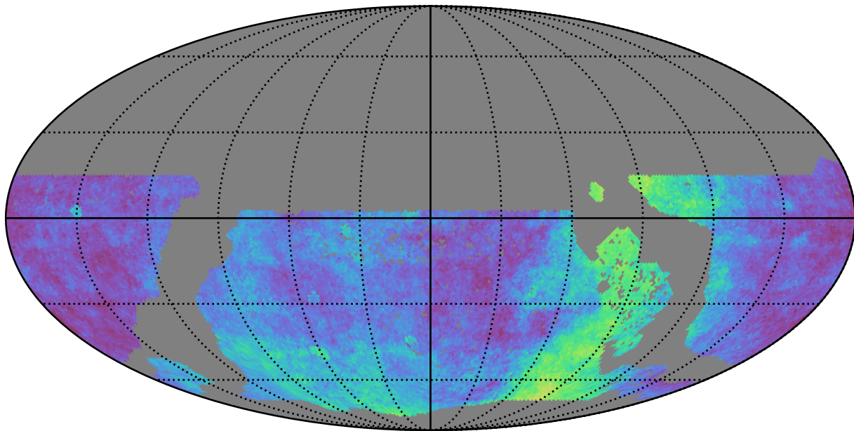
too_ignore_10_1v3.4_10yrs WFD: Parallax Coverage @ 24.0
