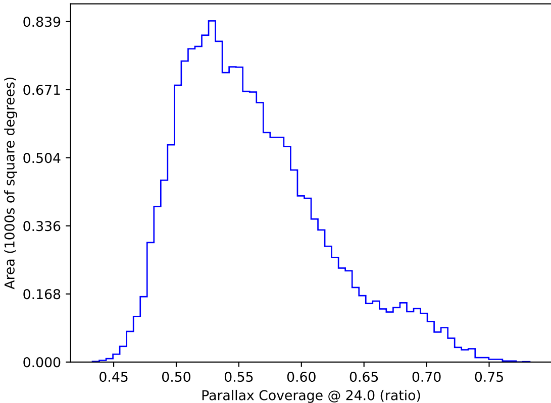
too_ignore_10_1v3.4_10yrs WFD: Parallax Coverage @ 24.0
