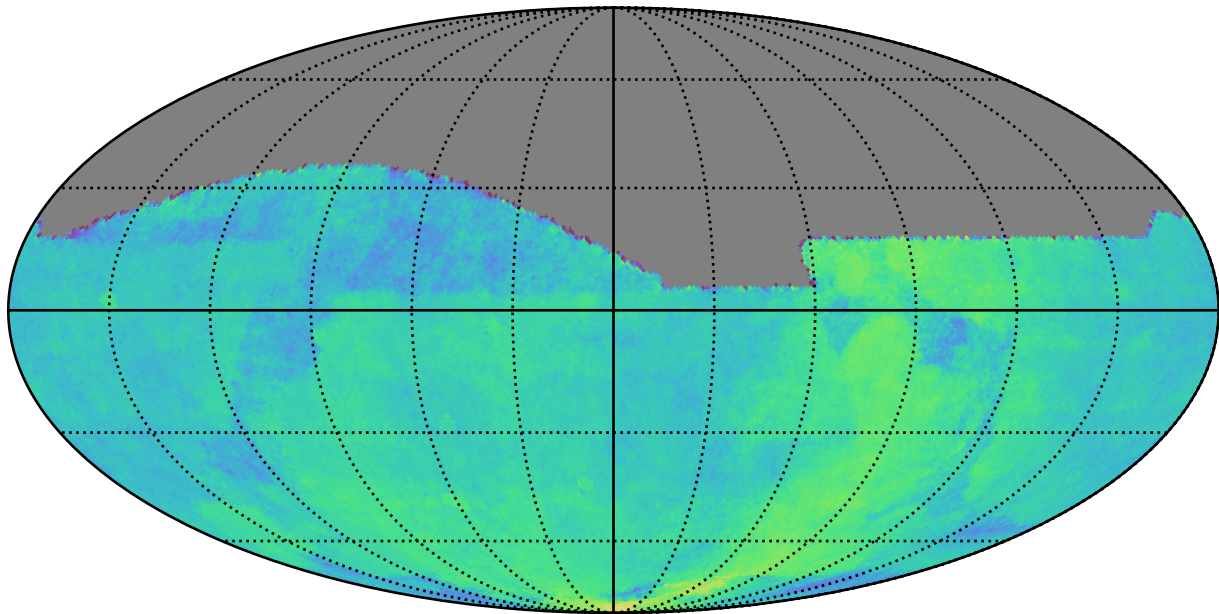
too_ignore_10_1v3.4_10yrs All sky: Parallax Coverage @ 24.0
