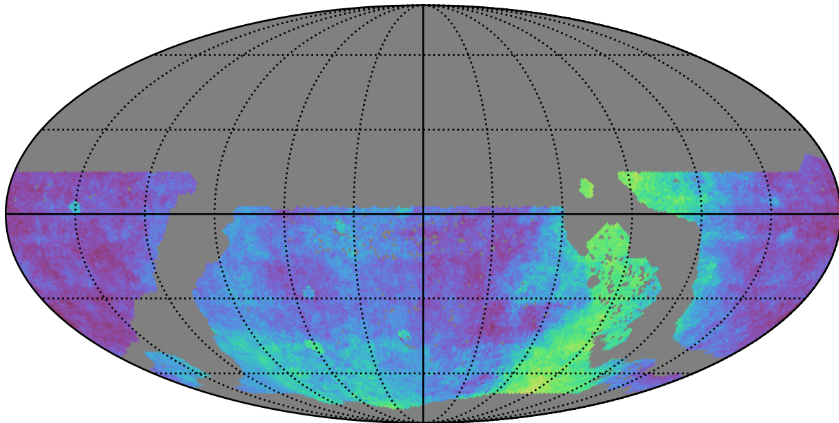
too_ignore_10_1v3.4_10yrs WFD: Parallax Coverage @ 22.4
