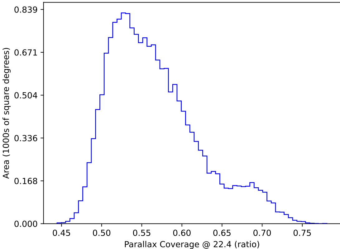
too_ignore_10_1v3.4_10yrs WFD: Parallax Coverage @ 22.4
