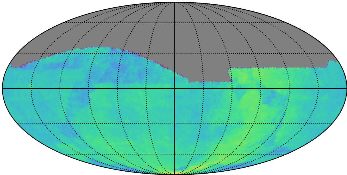
too_ignore_10_1v3.4_10yrs All sky: Parallax Coverage @ 22.4
