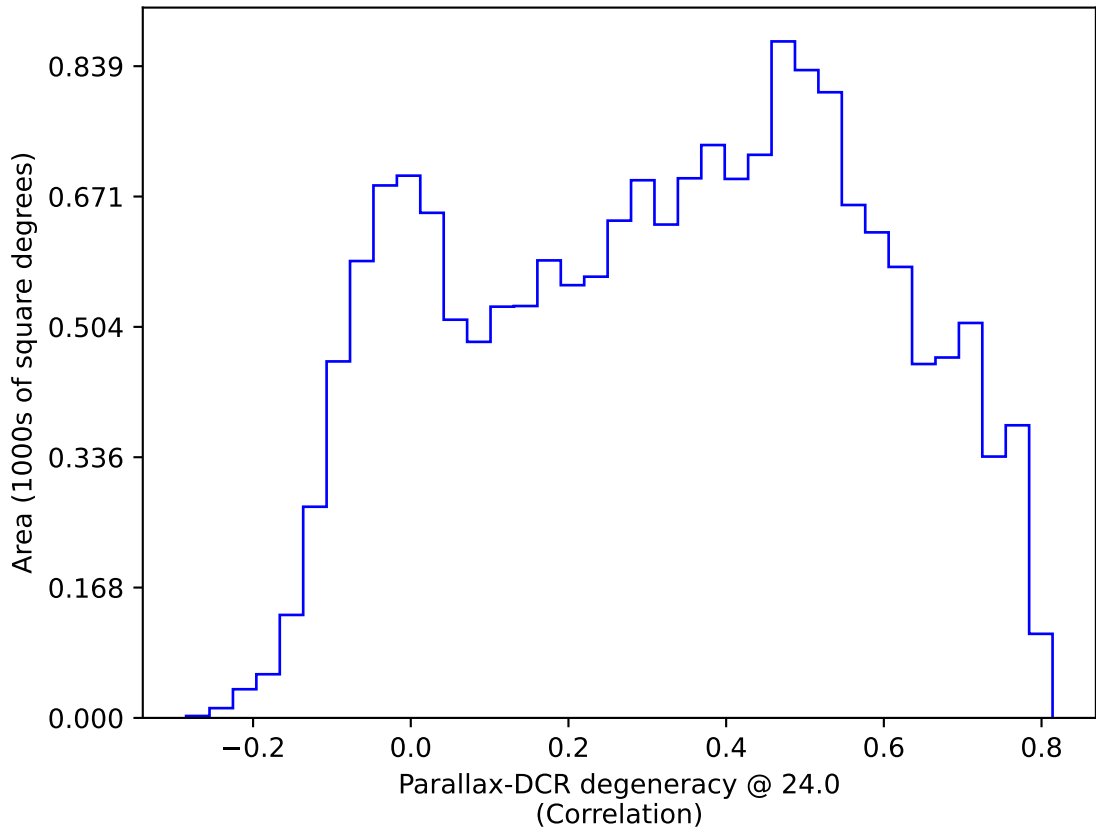
too_ignore_10_1v3.4_10yrs WFD: Parallax-DCR degeneracy @ 24.0
