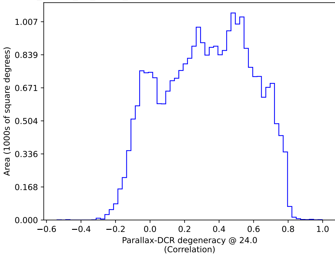
too_ignore_10_1v3.4_10yrs All sky: Parallax-DCR degeneracy @ 24.0
