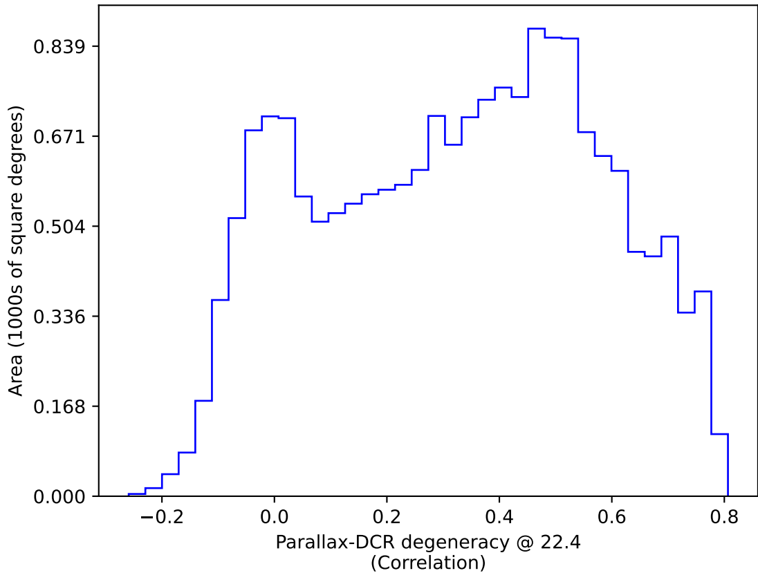
too_ignore_10_1v3.4_10yrs WFD: Parallax-DCR degeneracy @ 22.4
