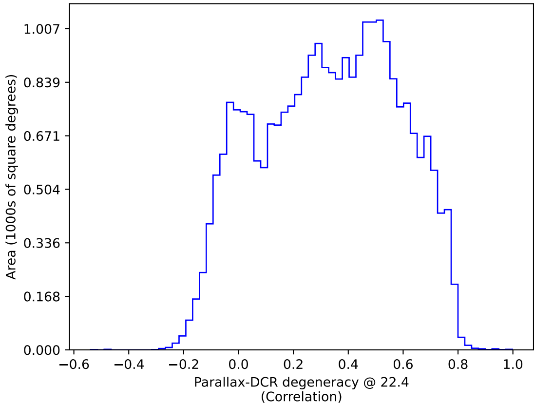
too_ignore_10_1v3.4_10yrs All sky: Parallax-DCR degeneracy @ 22.4
