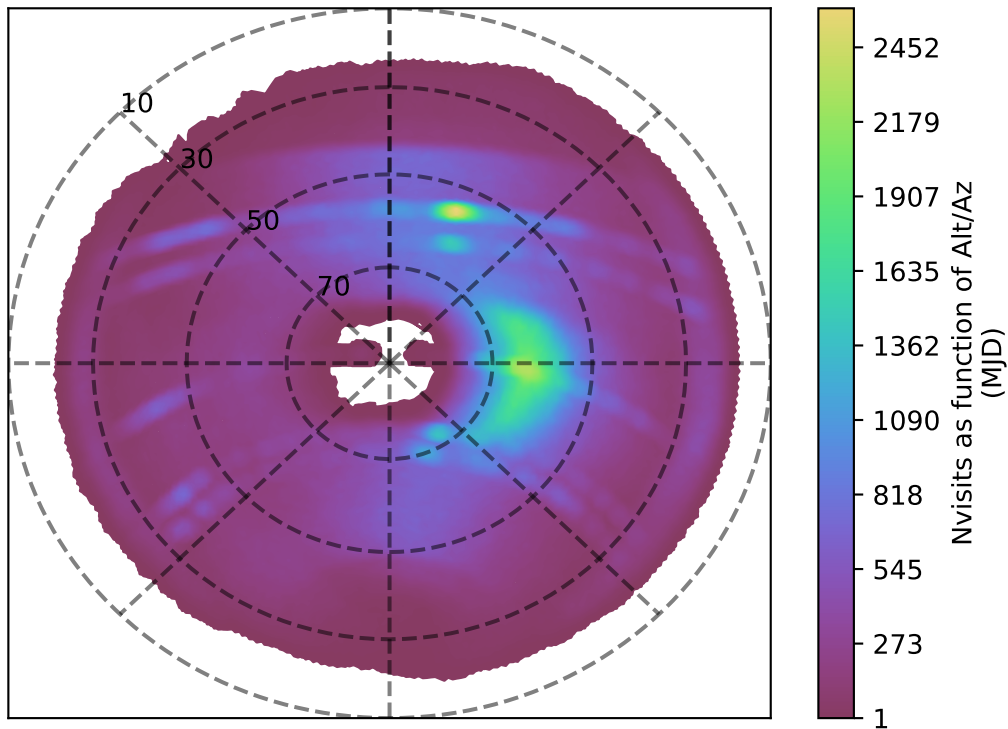
too_ignore_10_1v3.4_10yrs z band: Nvisits as function of Alt/Az
