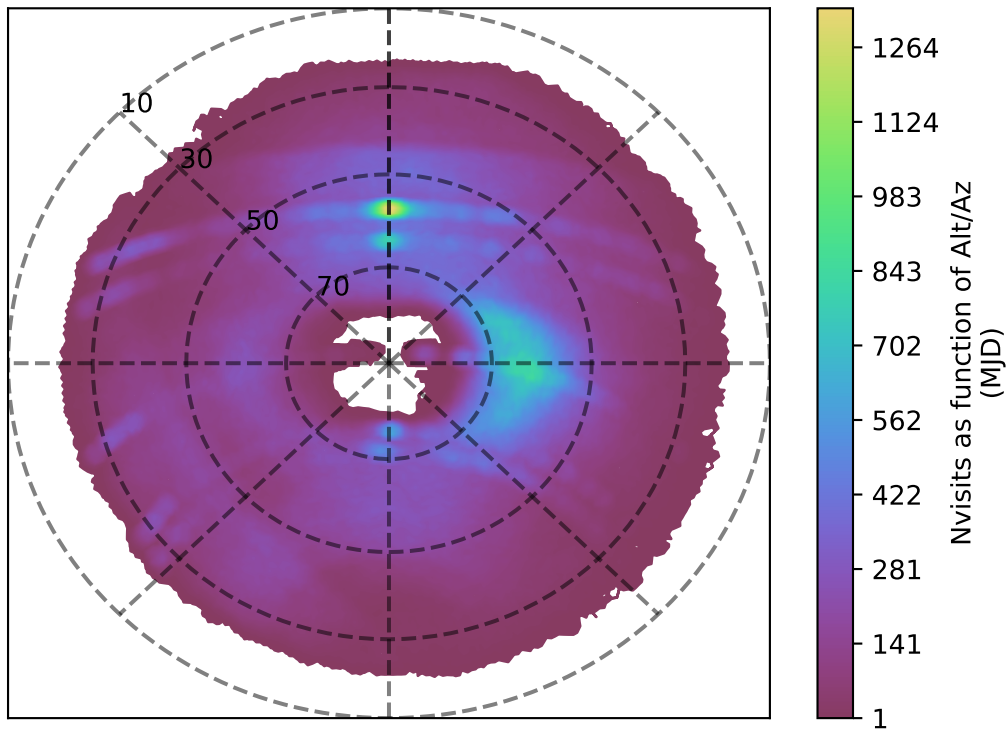
too_ignore_10_1v3.4_10yrs g band: Nvisits as function of Alt/Az
