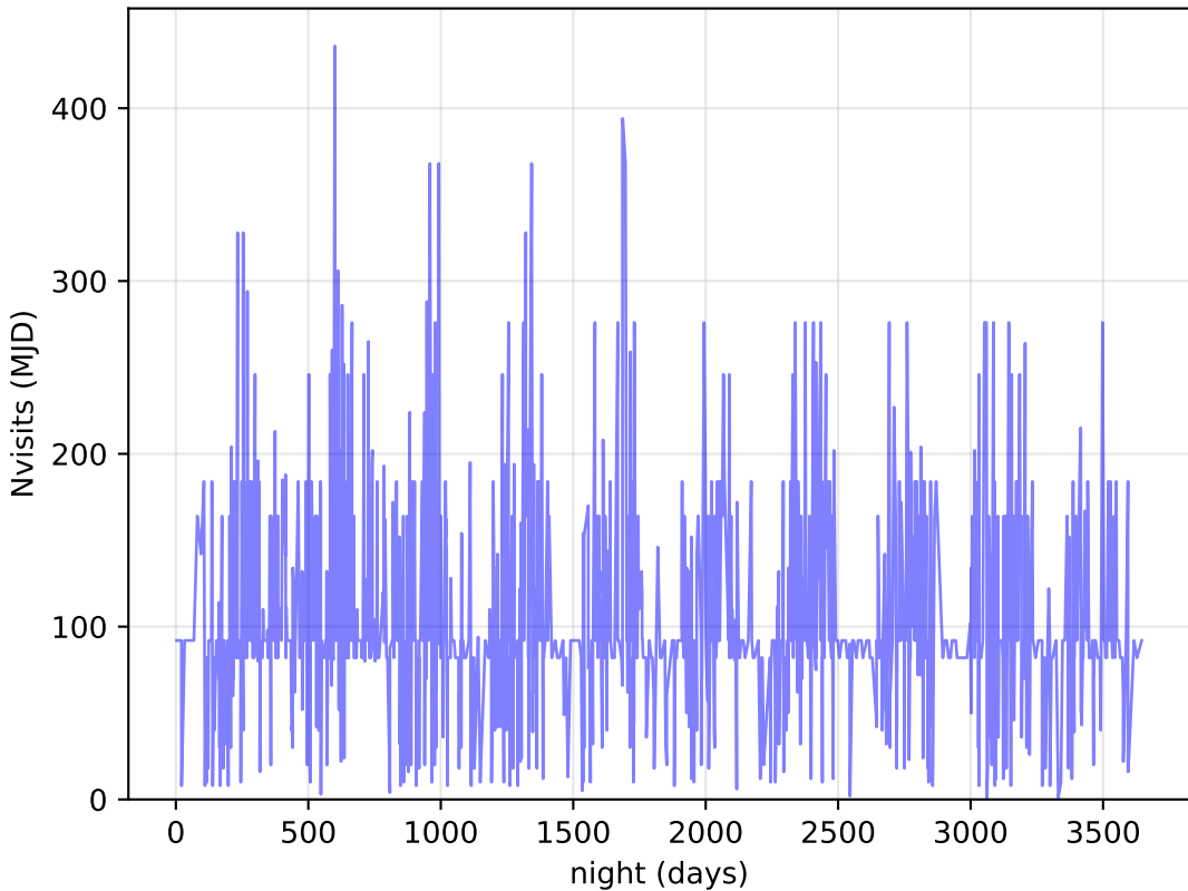
too_ignore_10_1v3.4_10yrs DDF: Nvisits
