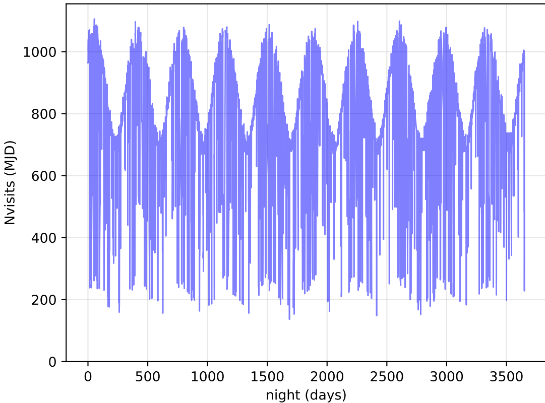
too_ignore_10_1v3.4_10yrs All visits: Nvisits
