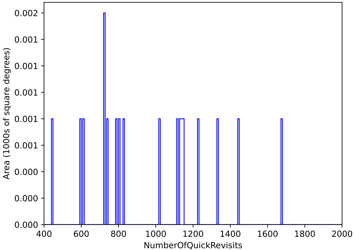
too_ignore_10_1v3.4_10yrs WFD: NumberOfQuickRevisits
