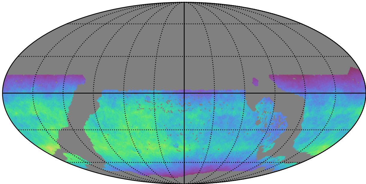
too_ignore_10_1v3.4_10yrs WFD y band: Normalized Teff
