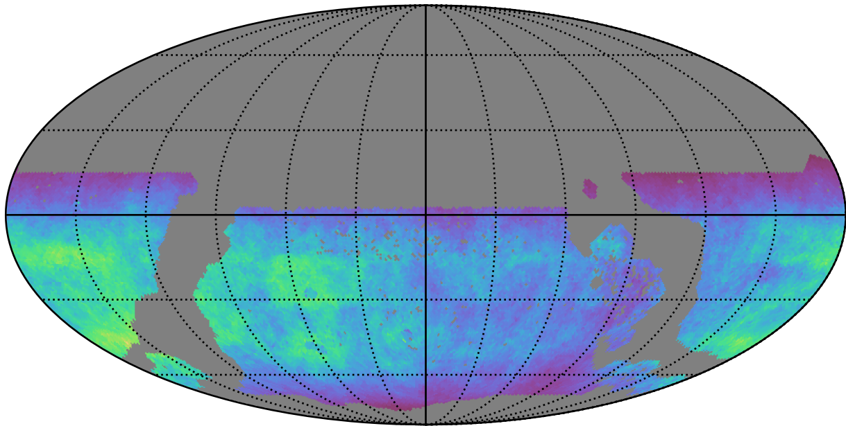
too_ignore_10_1v3.4_10yrs WFD u band: Normalized Teff
